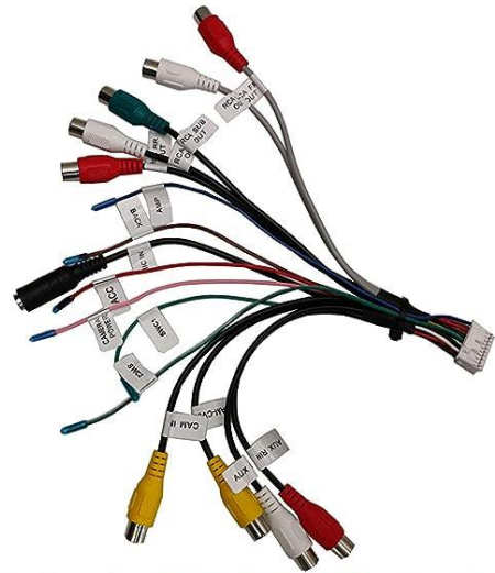
Kabelbund: (AUX-IN, CAM-IN, Mikrophon-IN, SUB-OUT, 4 x Audio-Out, ACC, Kamera Power, Back, AMP)
