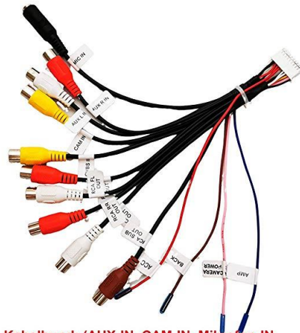
Kabelbund: (AUX-IN, CAM-IN, Mikrofon-IN, SUB-OUT, 4 x Audio-Out, ACC, Kamera Power, Back, AMP)
