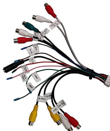
Kabelbund: (AUX-IN, CAM-IN, Mikrofon-IN, SUB-OUT, 4 x Audio-Out, ACC, Kamera Power, Back, AMP)
